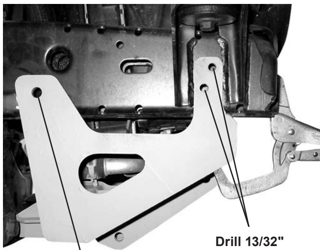
Drill 17/32" holes.
